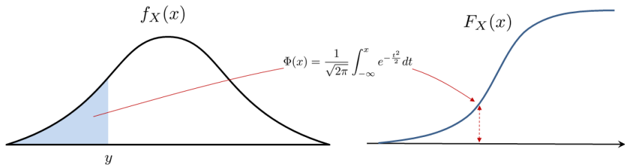
Figure: Definition of the CDF of the standard Gaussian \Phi(x) .
